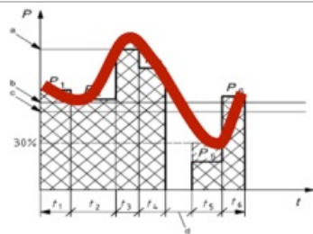
Variable Load
