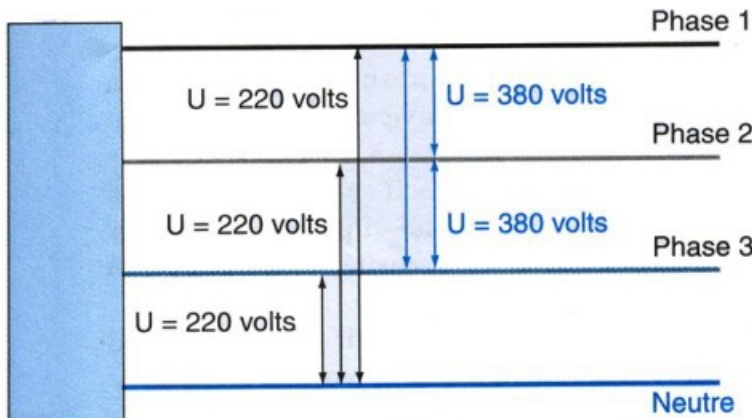
Three-Phase
